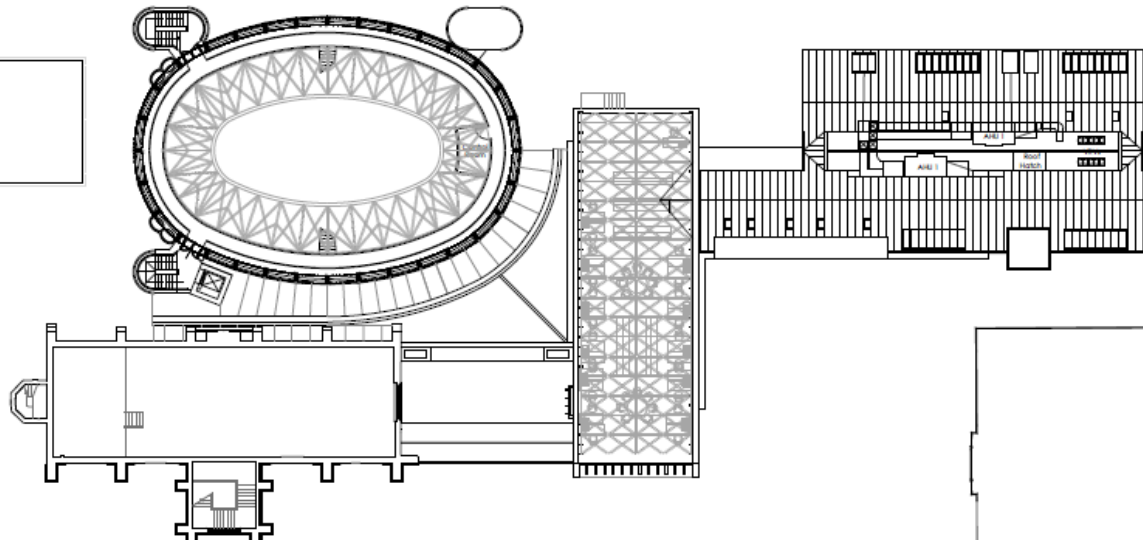
Technical Level Floor Plan
